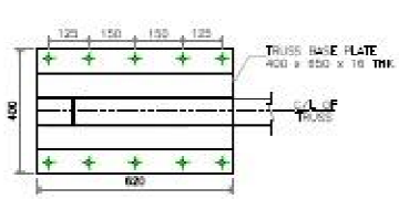
DETAILS OF COLUMN CAP PLATE
