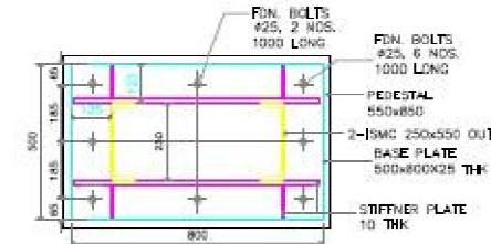
BOLT DETAILS
