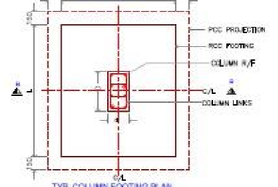
TYP. COLUMN FOOTING PLAN
