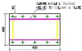
DETAILS OF COLUMN CAP PLATE
