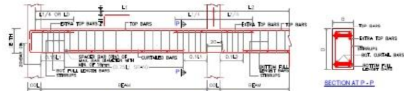
TYP LONGITUDINAL SECTION OF BEAM
