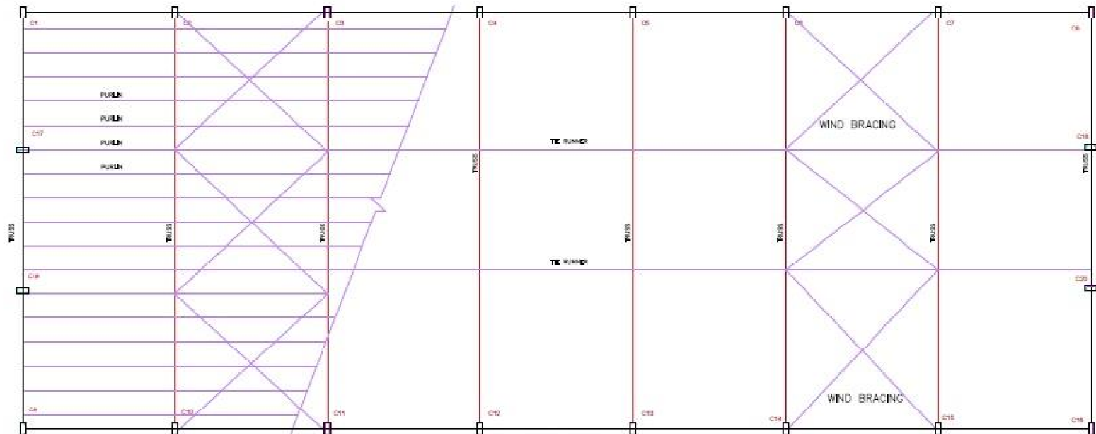
PLAN AT TRUSS TIE LVL
