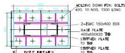
BOLT DETAILS
